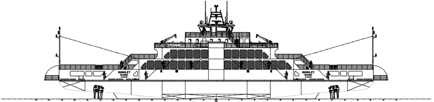
PROFILE VIEW
