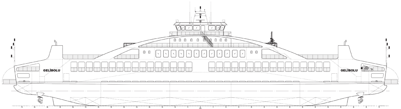
PROFILE VIEW
