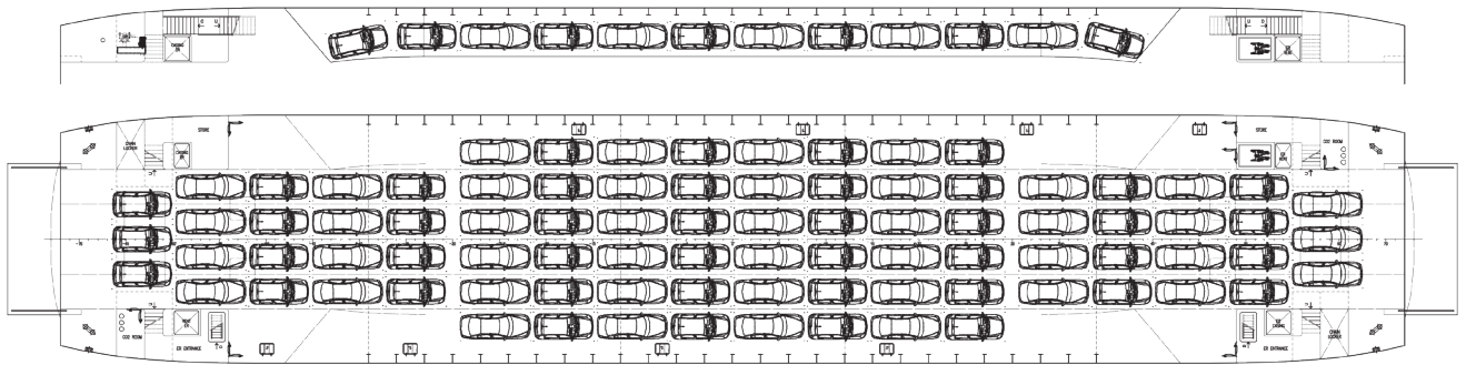
CAR DECK
