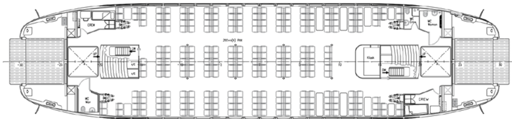
Main Deck 3000 mm x 19 m B.L.
