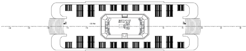
Bridge Deck 8175 mm x 19 m B.L.
