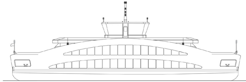
PROFILE VIEW
